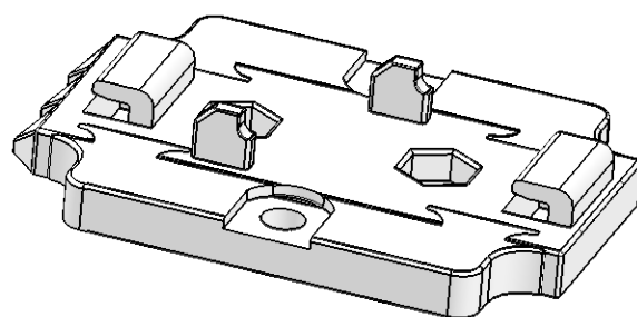
4532000100 Simco standard mounting bracket
